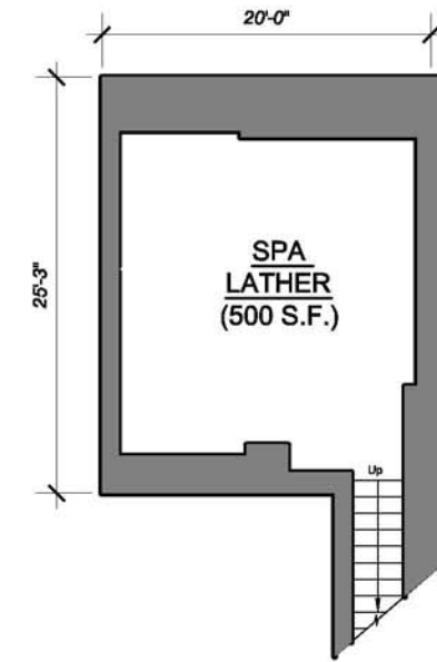
LOWER LEVEL PLAN
